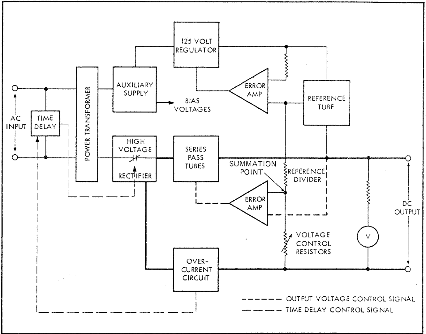
Figure 3-1. MODEL 415B BLOCK DIAGRAM
