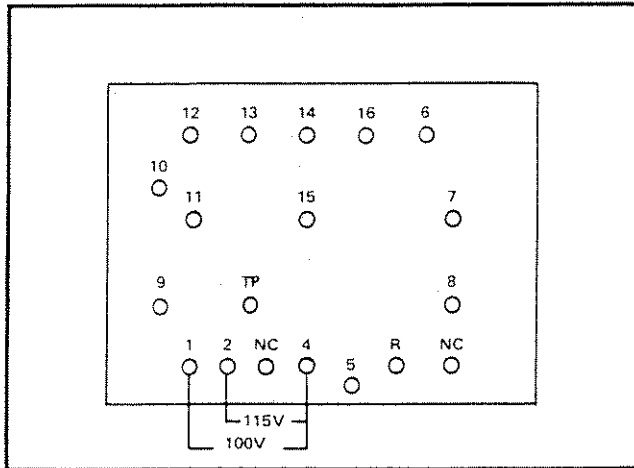
Figure 2-2. POWER TRANSFORMER TERMINALS
