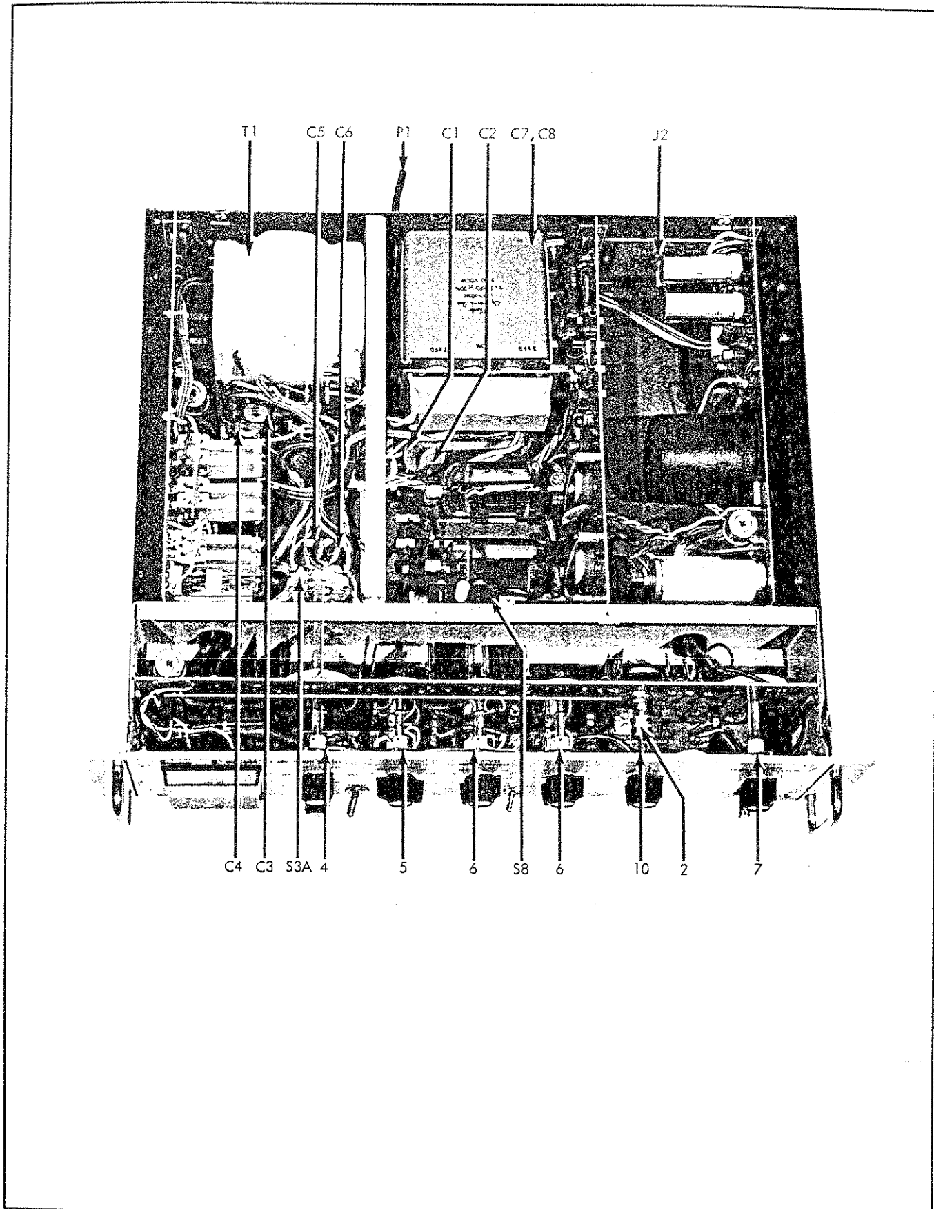
Figure 5-2. CHASSIS ASSEMBLY
