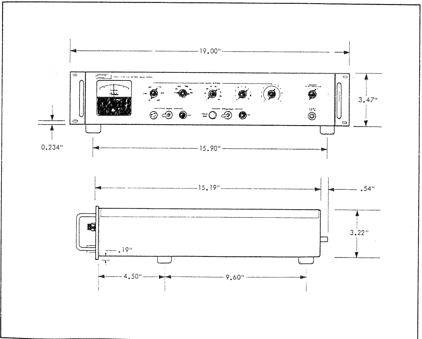
Figure 1-1. MODEL 415B OUTLINE DRAWING
