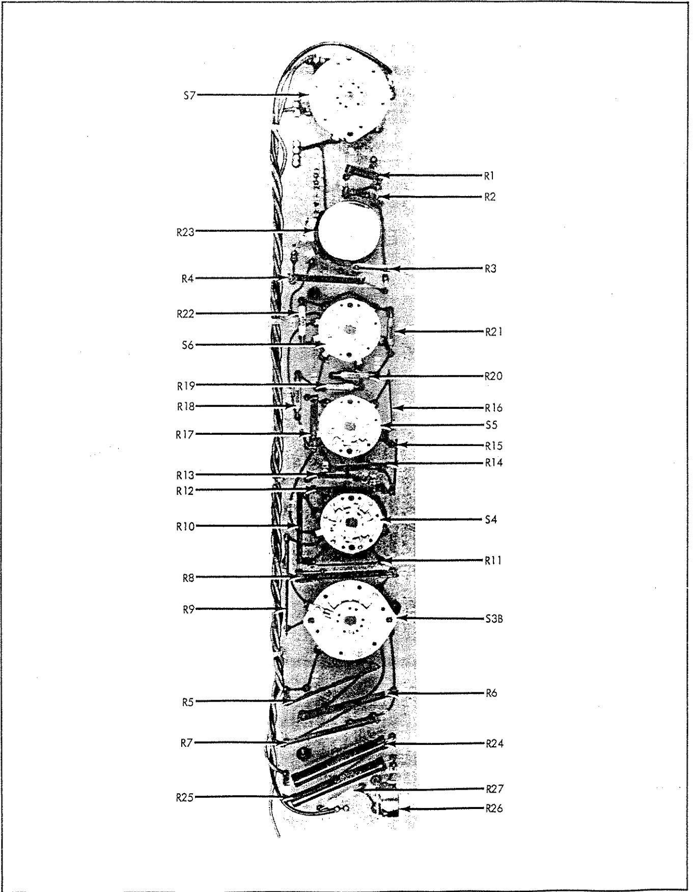
Figure 5-4. SWITCH P/C ASSEMBLY
