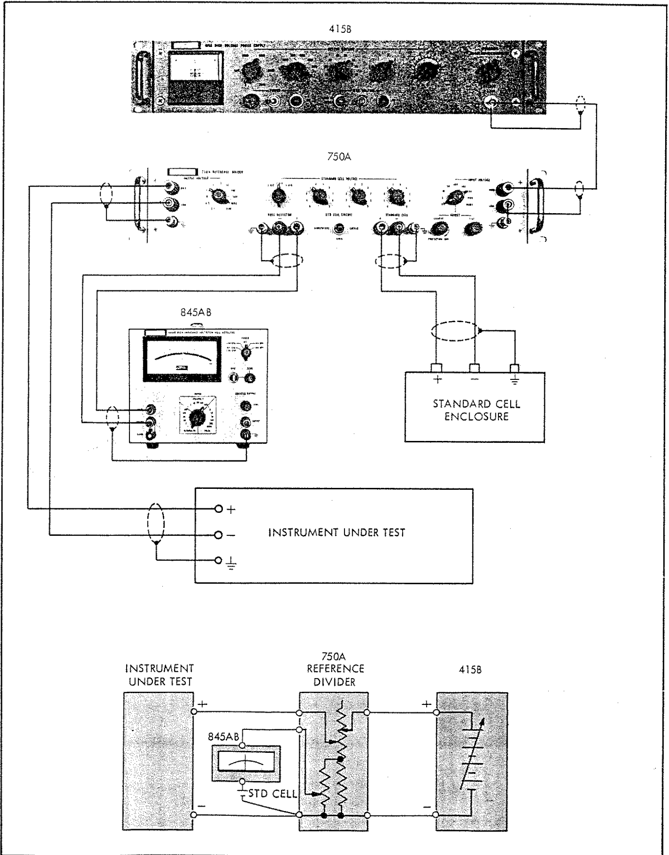
Figure 2-3. OPERATION WITH A REFERENCE DIVIDER
