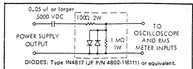
Figure 4-2. PROTECTION CIRCUIT
