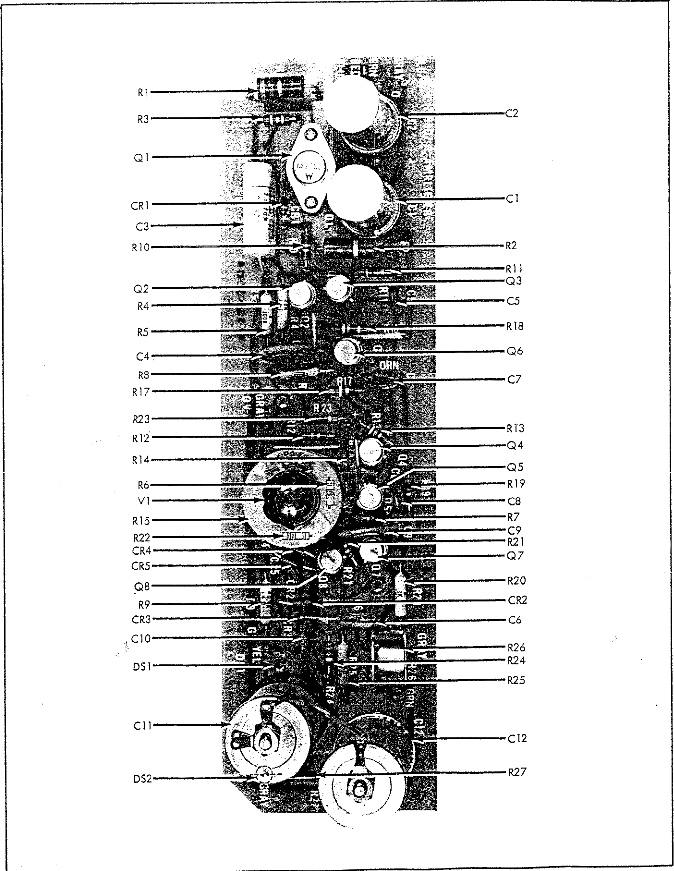
Figure 5-7. AMPLIFIER P/C ASSEMBLY
