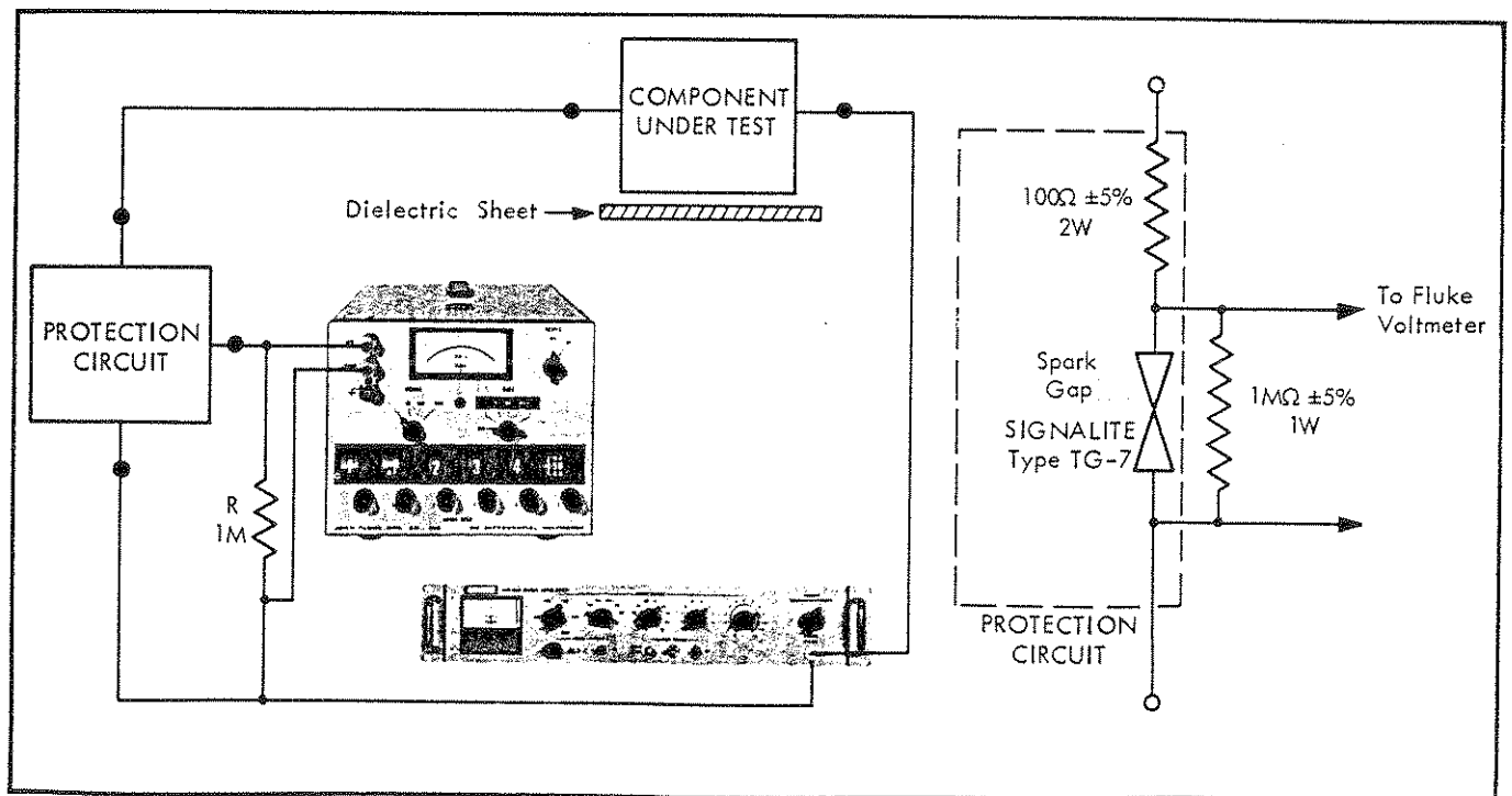
Figure 2-4. LEAKAGE CURRENT TESTING
