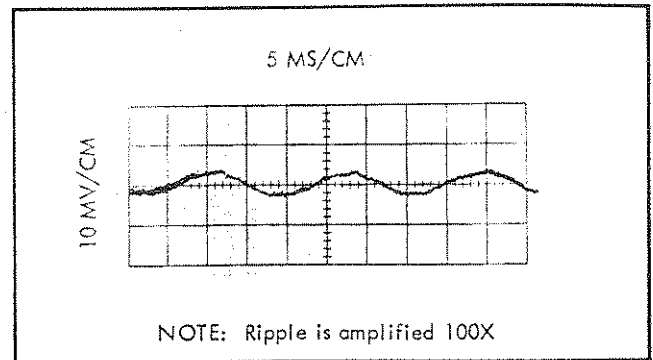
Figure 4-5. RIPPLE ON HIGH VOLTAGE DC OUTPUT
