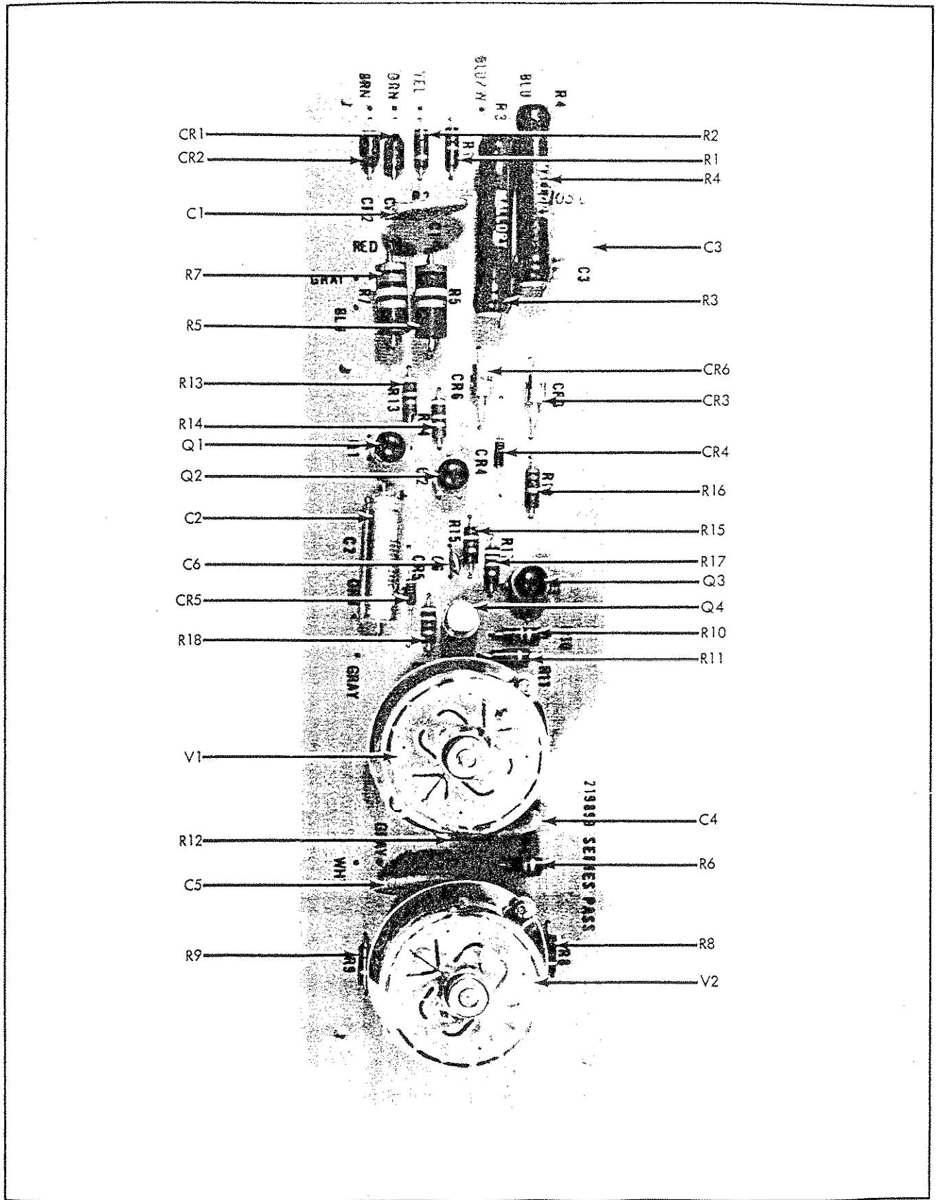
Figure 5-6. SERIES PASS P/C ASSEMBLY
